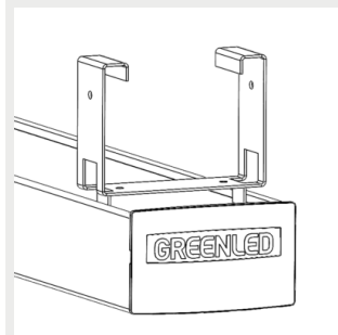
E1500147 Suspension rail bracket MEK 82 white
