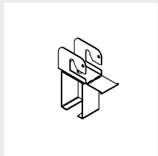
3508141 Bracket for Horizontal Wire
