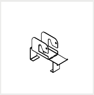
3508009 Horizontal wire bracket
