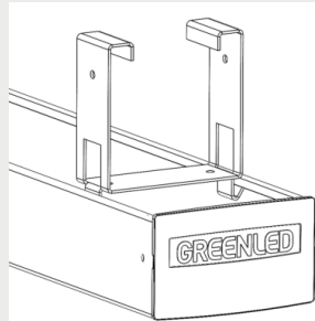
9908435 Suspension rail bracket MEK 70
