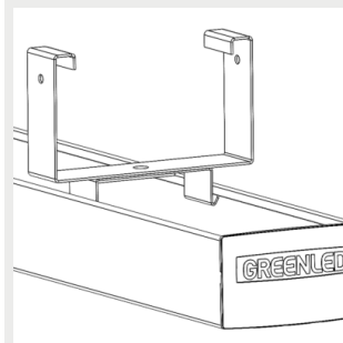
E1500149 Suspension rail bracket MEK 110 white
