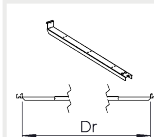
Omega/ALG2 railbracket (4)
