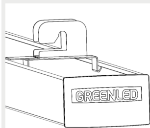
3508103 Horizontal wire bracket max 8 mm
