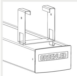
9908435 Suspension rail bracket MEK 70
